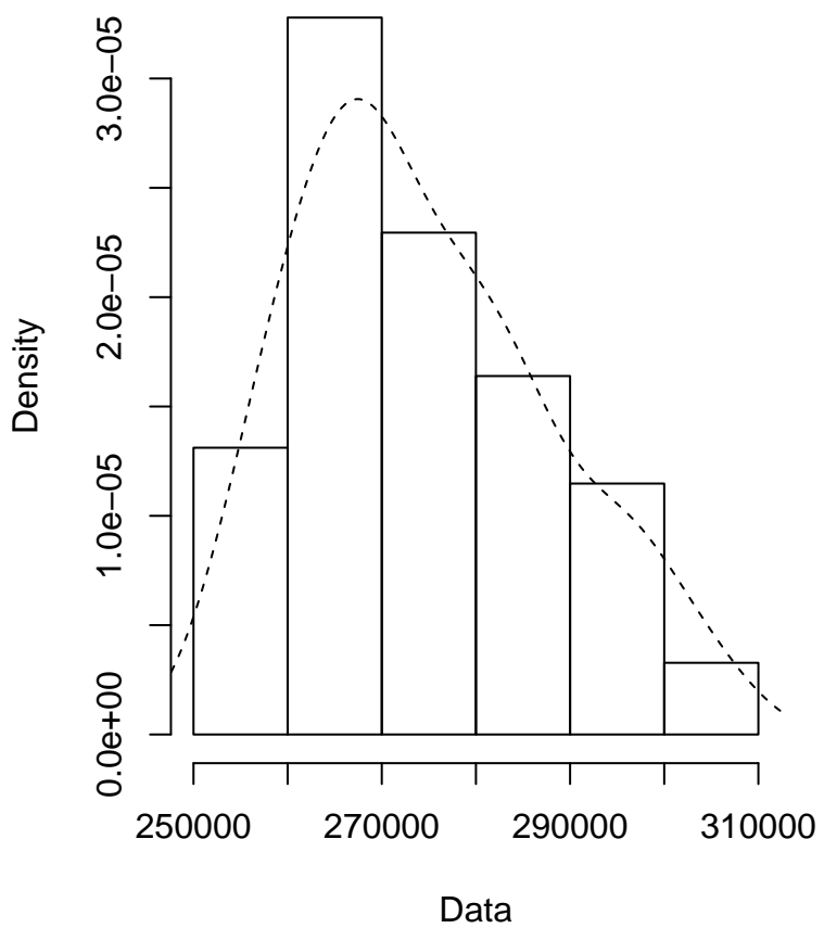
Empirical density
