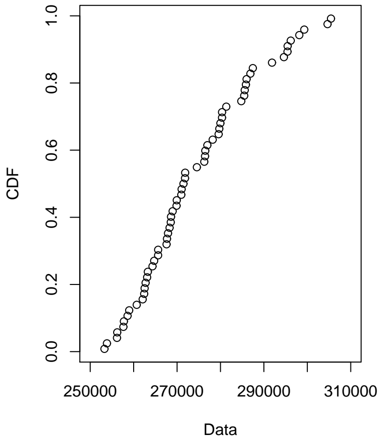
Cumulative distribution
