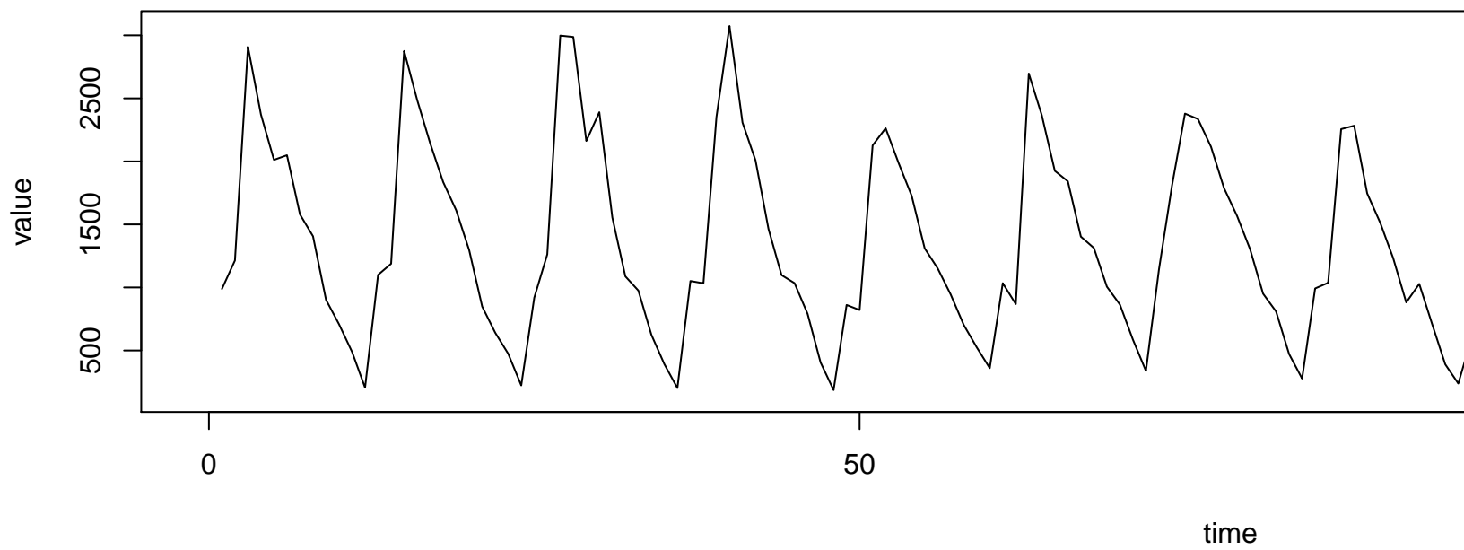
Working Time Series ( \lambda=1, d=0 )
