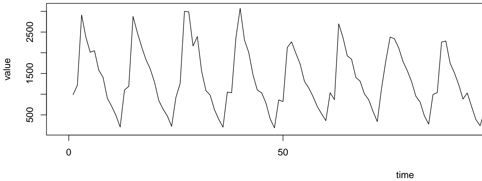
Original Time Series
