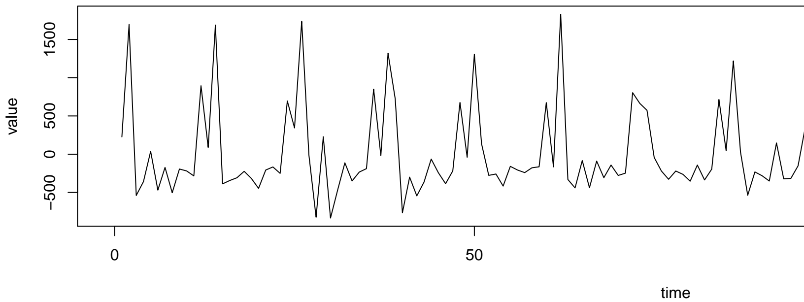
Working Time Series ( \lambda=1 , d=1 )
