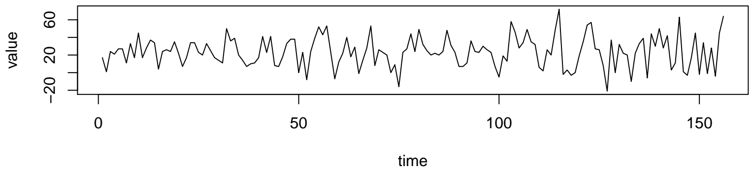
Working Time Series ( \lambda=1 , d=0 , D=1 )
