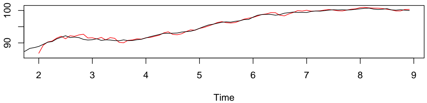
Interpolation Fit of Exponential Smoothing
