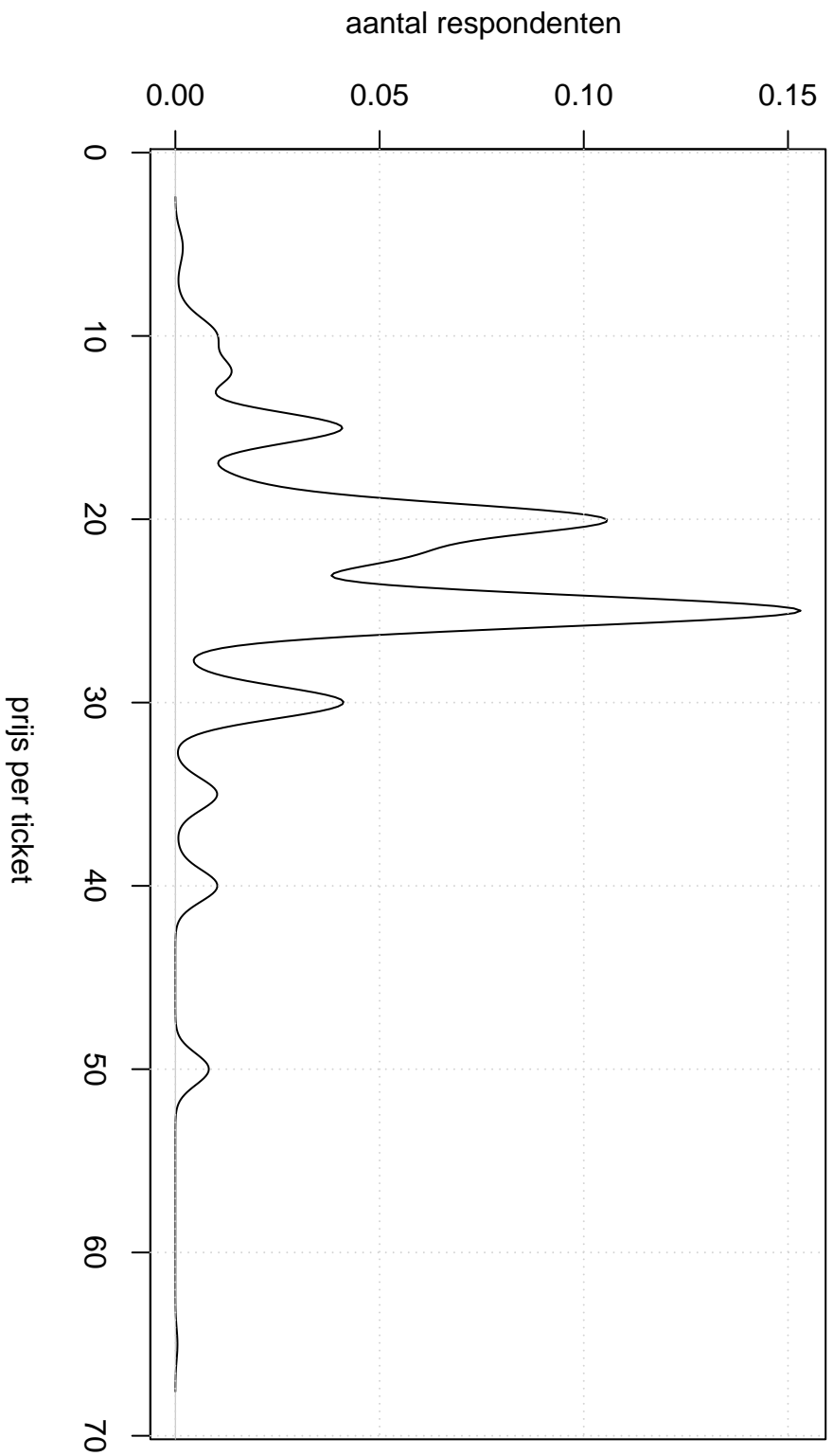
Gaussian Kernel
