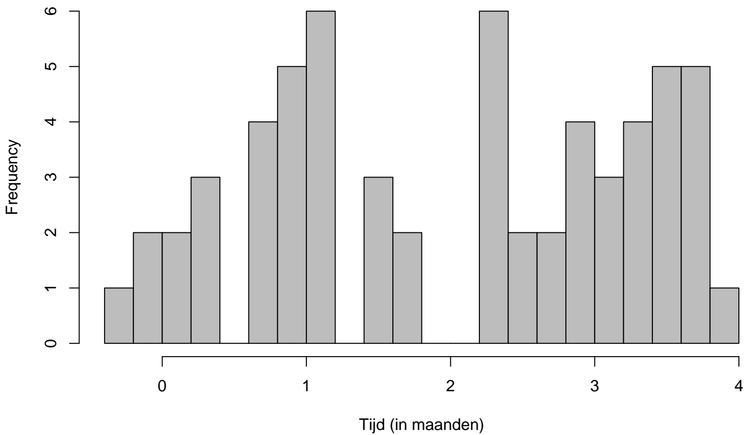
Histogram NCIP (2010–2014)
