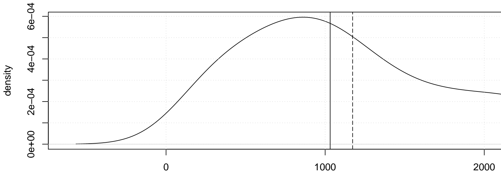
Density Plot – Gaussian Kernel
