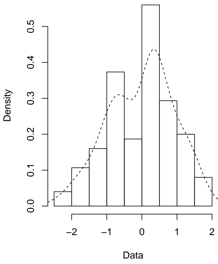
Empirical density
