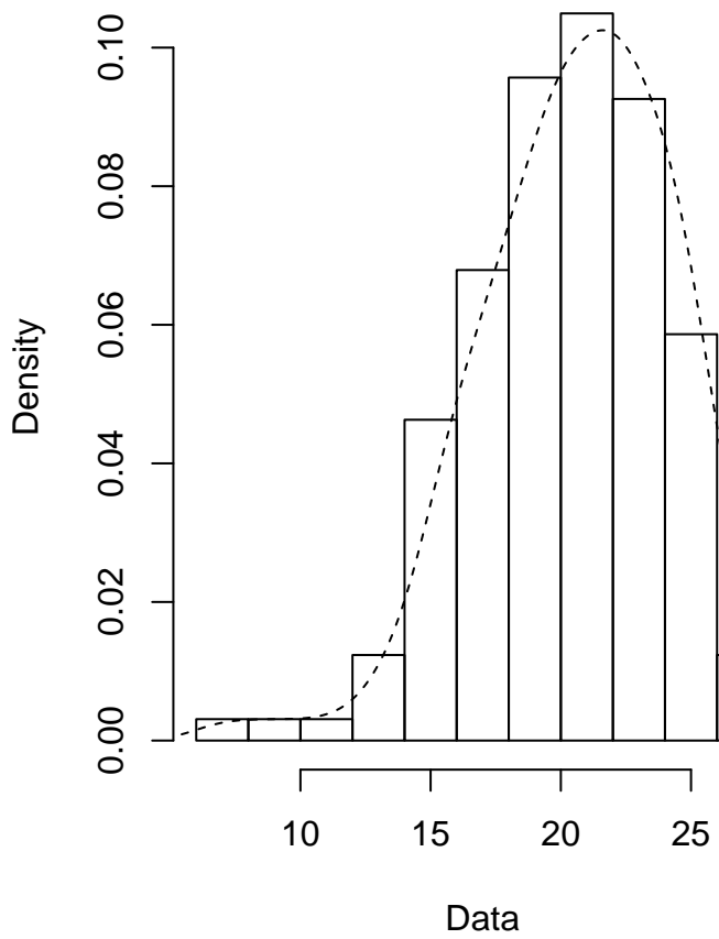
Empirical density
