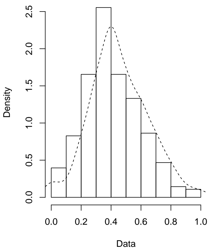
Empirical density
