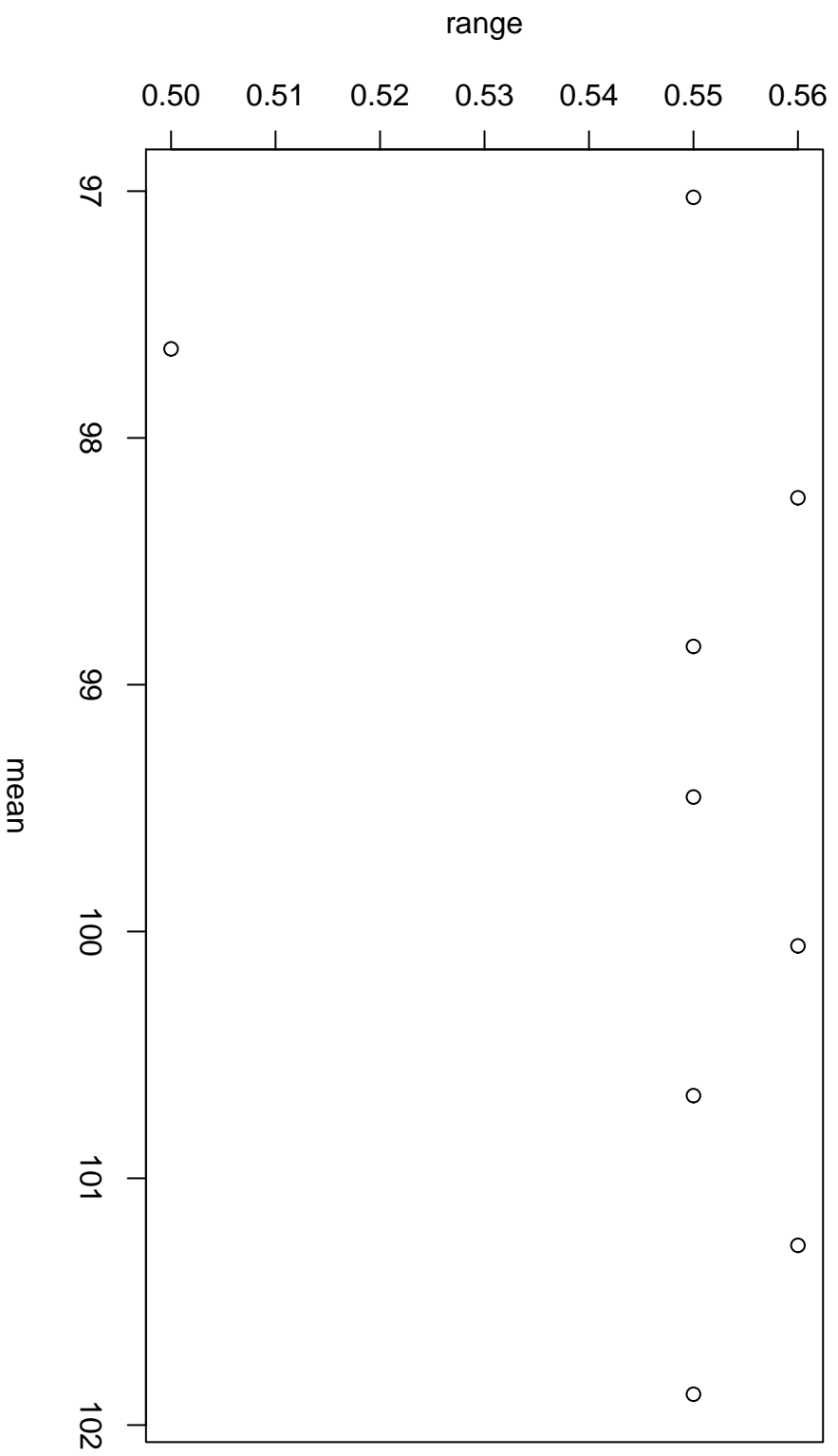
Range-Mean Plot
