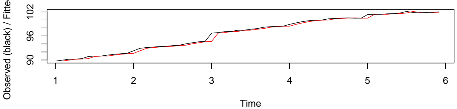
Interpolation Fit of Exponential Smoothing
