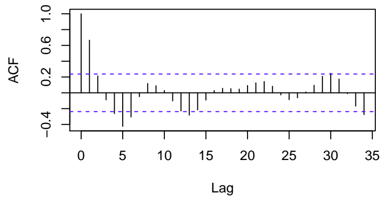
Random
