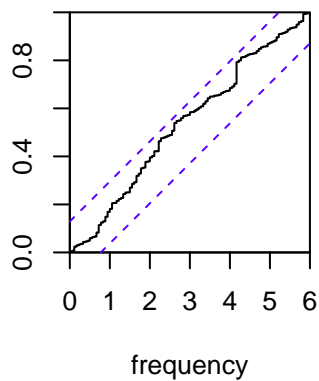
Residual Cumulative Periodogram
