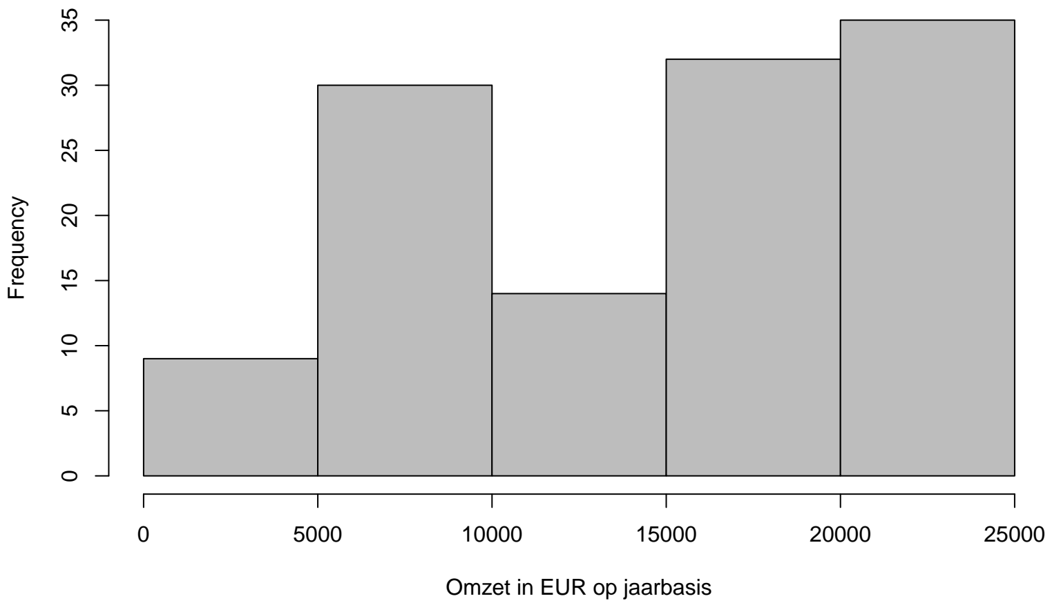
Histogram webcam
