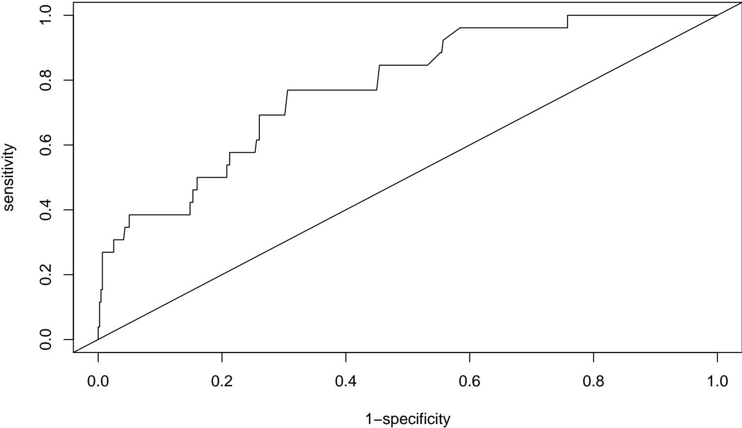
ROC plot
