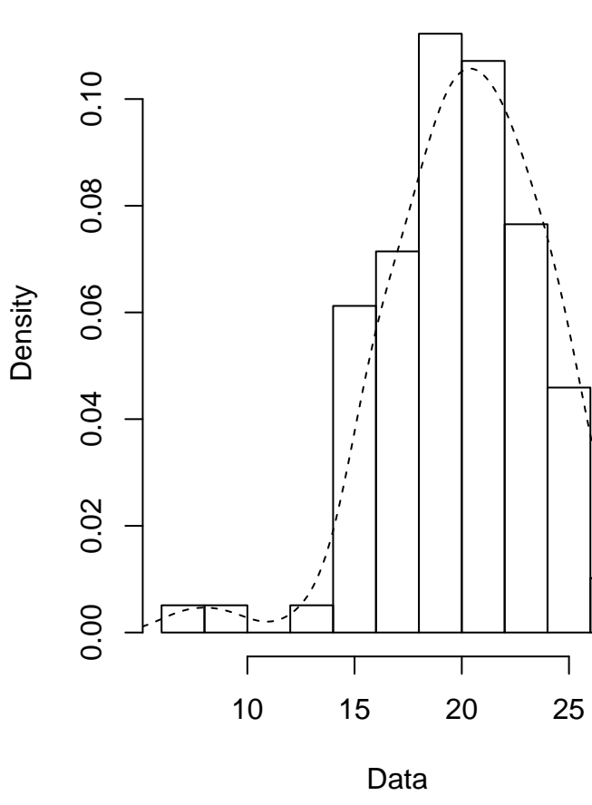
Empirical density
