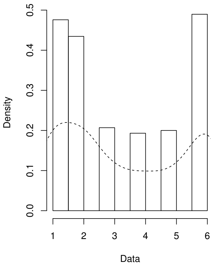
Empirical density
