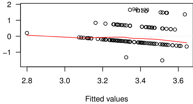
Residuals vs Fitted
