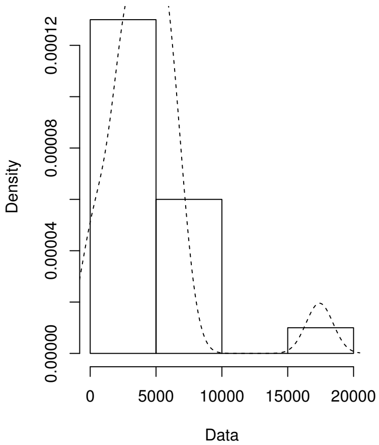
Empirical density
