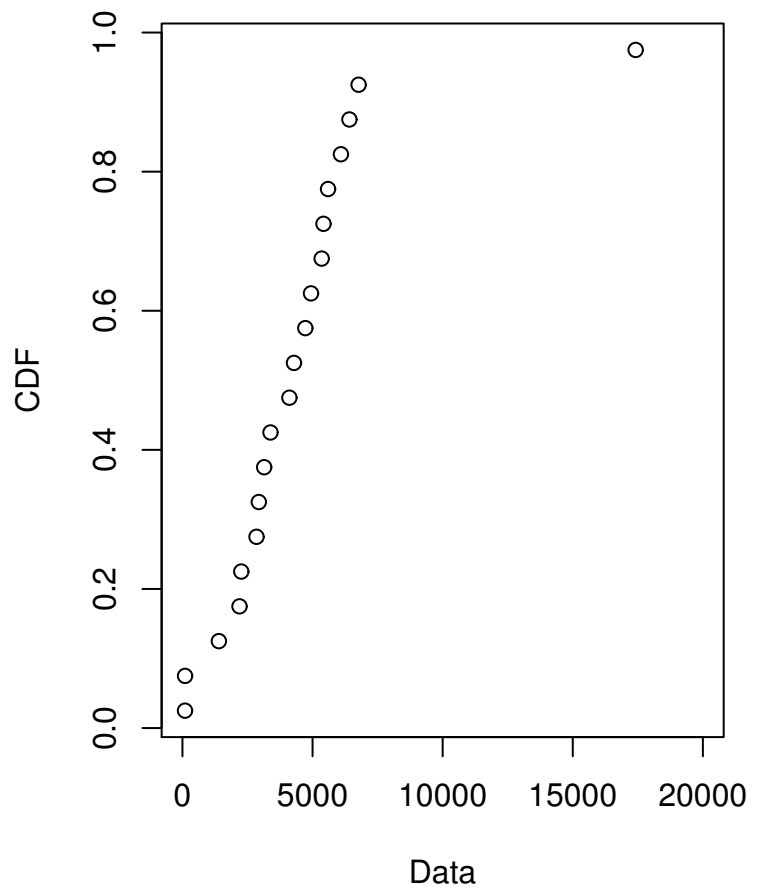
Cumulative distribution
