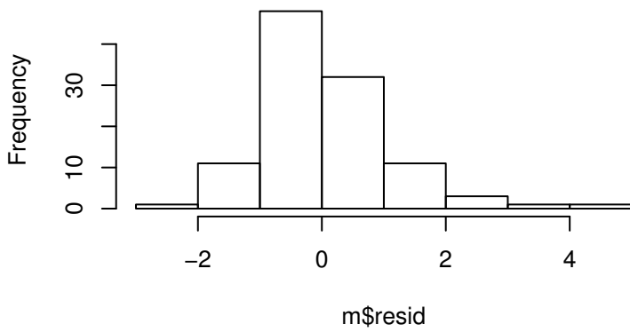
Residual Histogram
