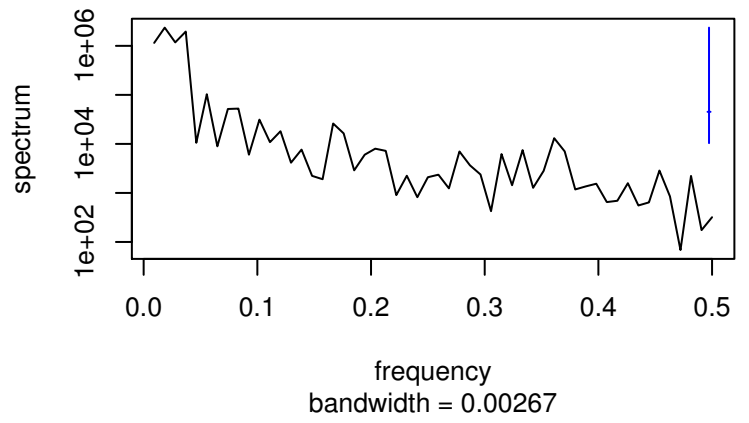
Standardized Residuals
