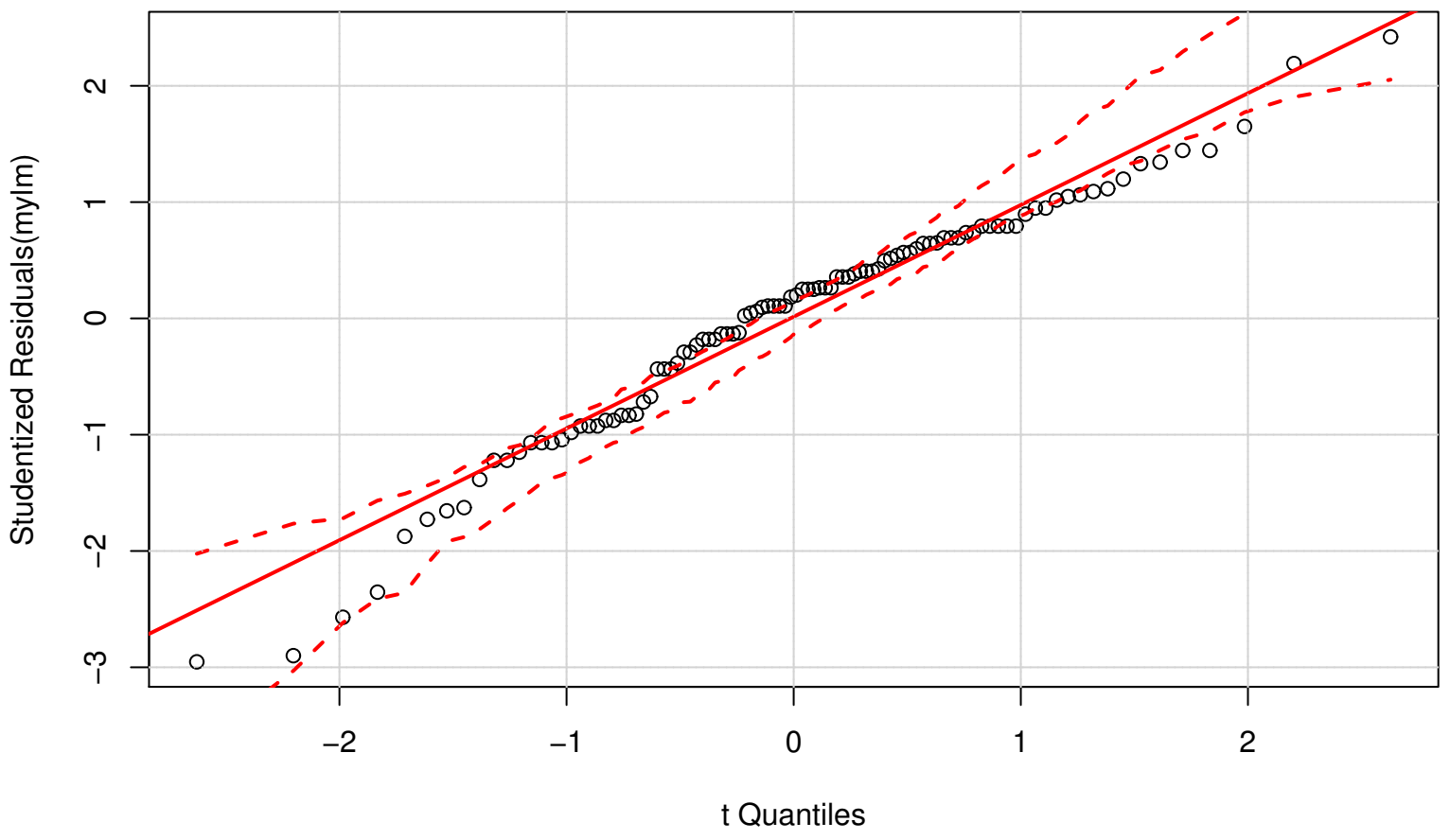
QQ Plot
