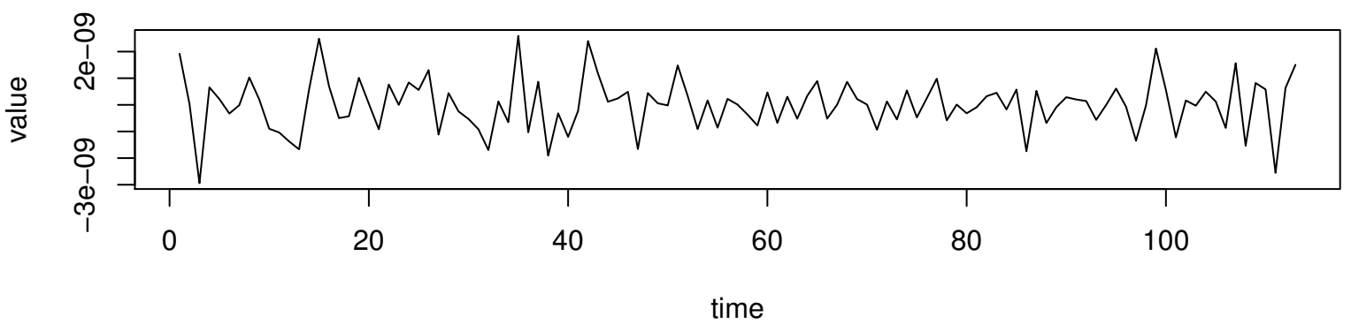
Working Time Series ( \lambda=-2 , d=1 , D=1 )
