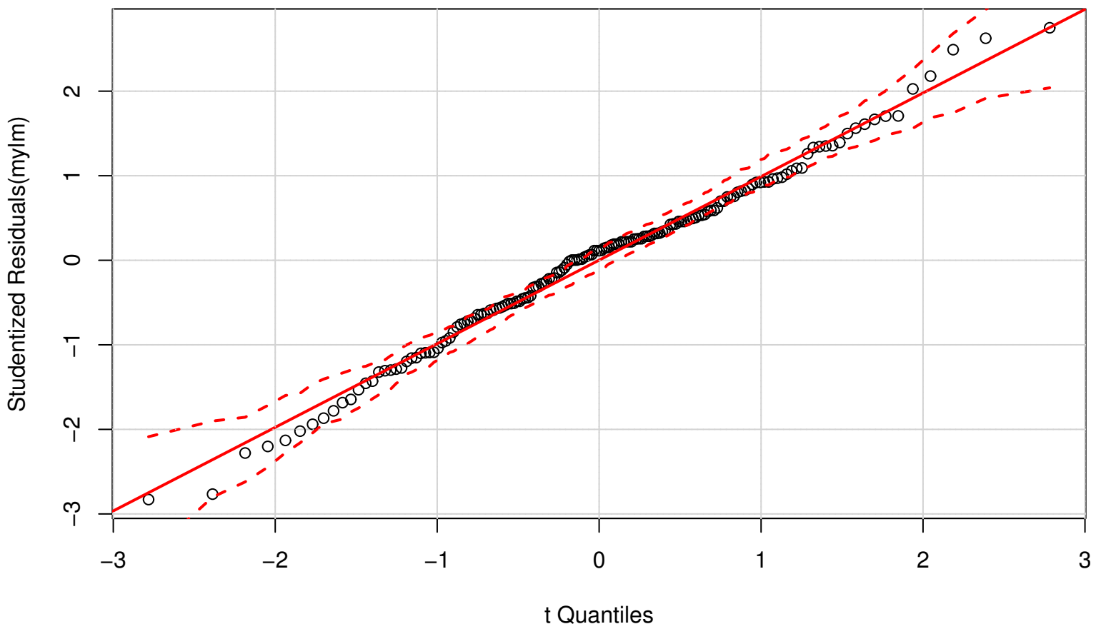
QQ Plot
