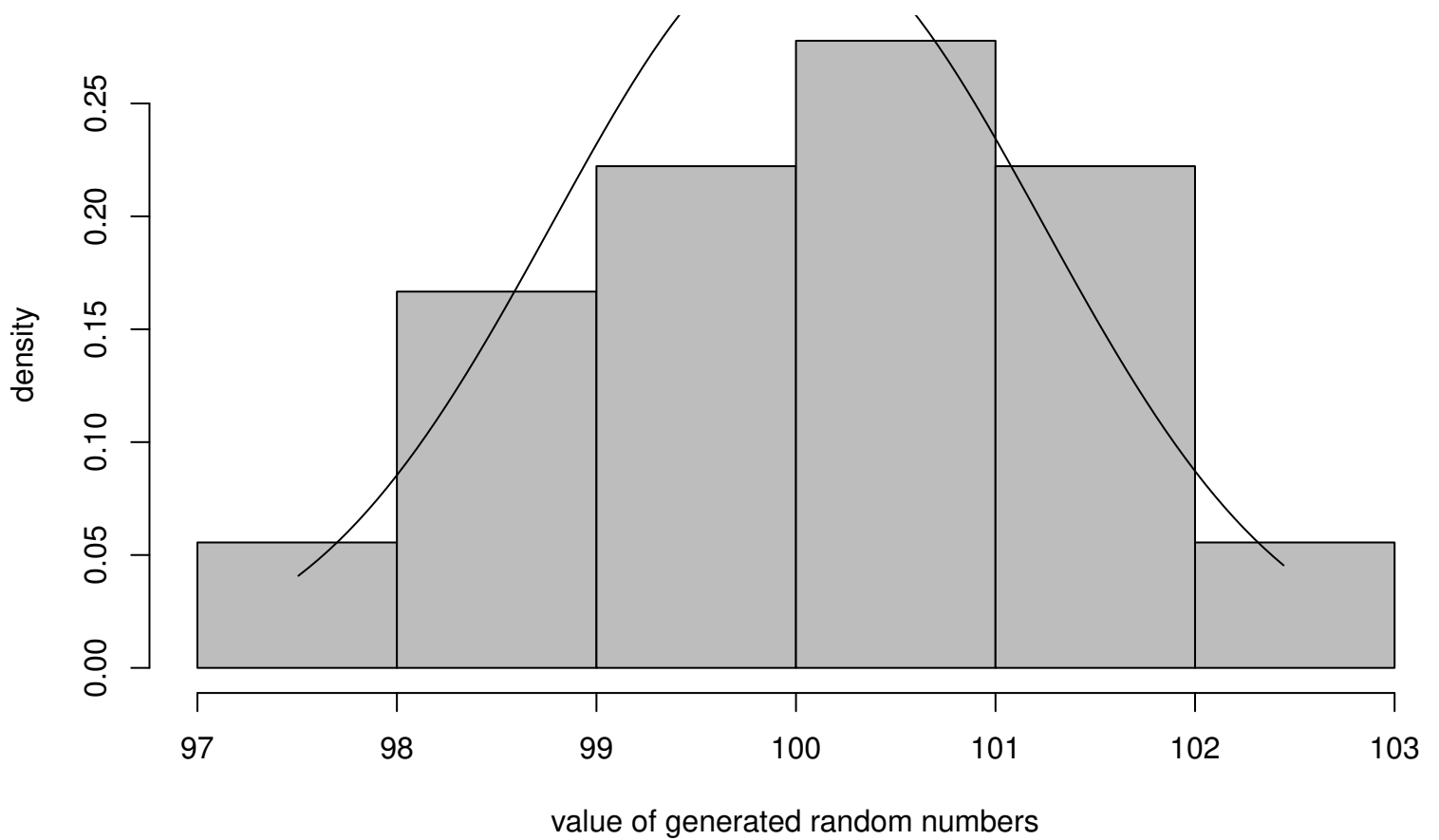
Histogram of Generated Random Numbers
