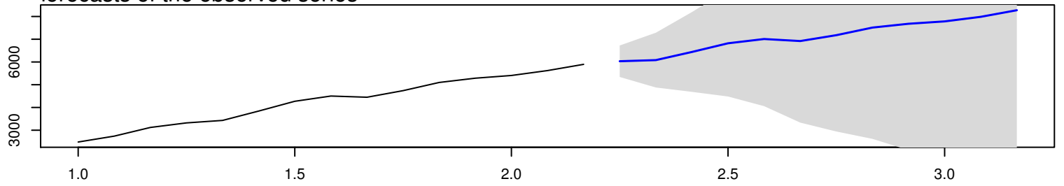
forecasts of the observed series
