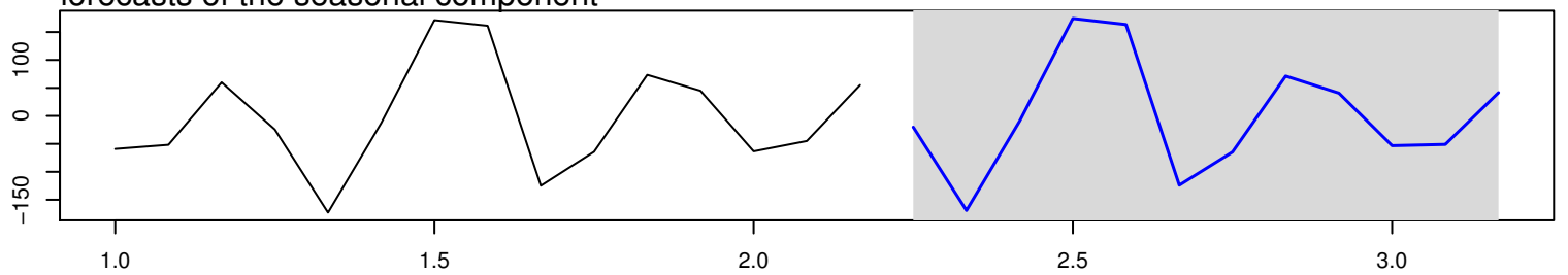
forecasts of the seasonal component
