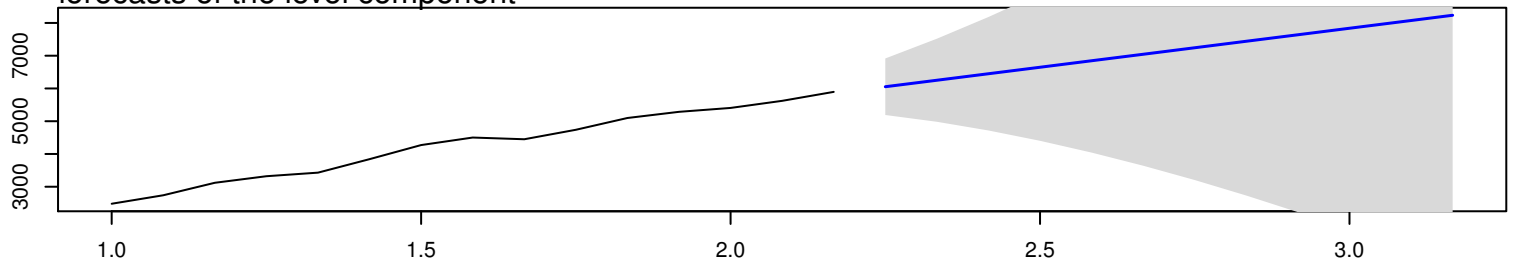
forecasts of the level component
