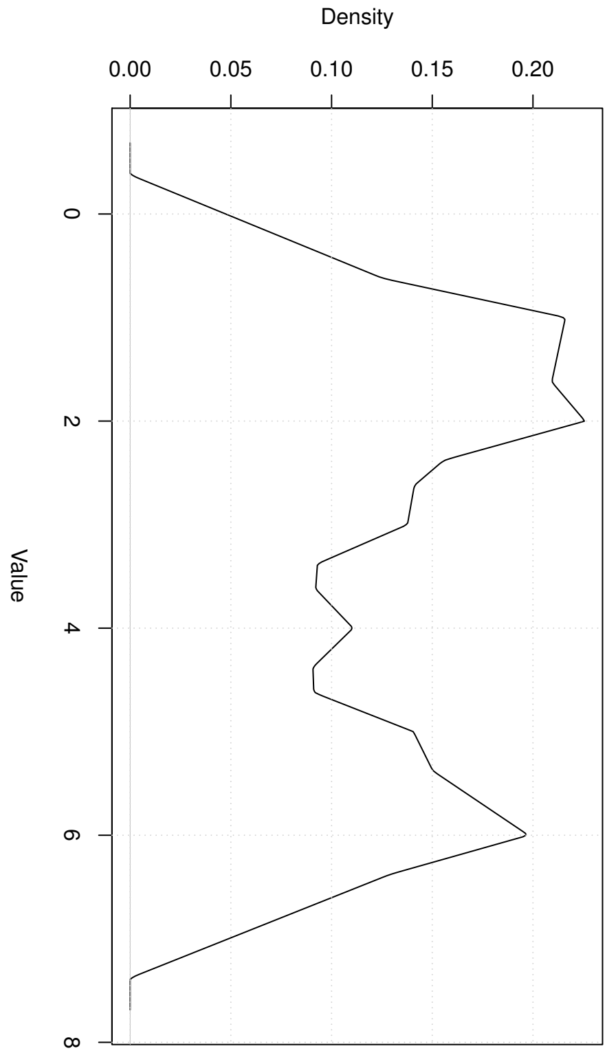
Triangular Kernel
