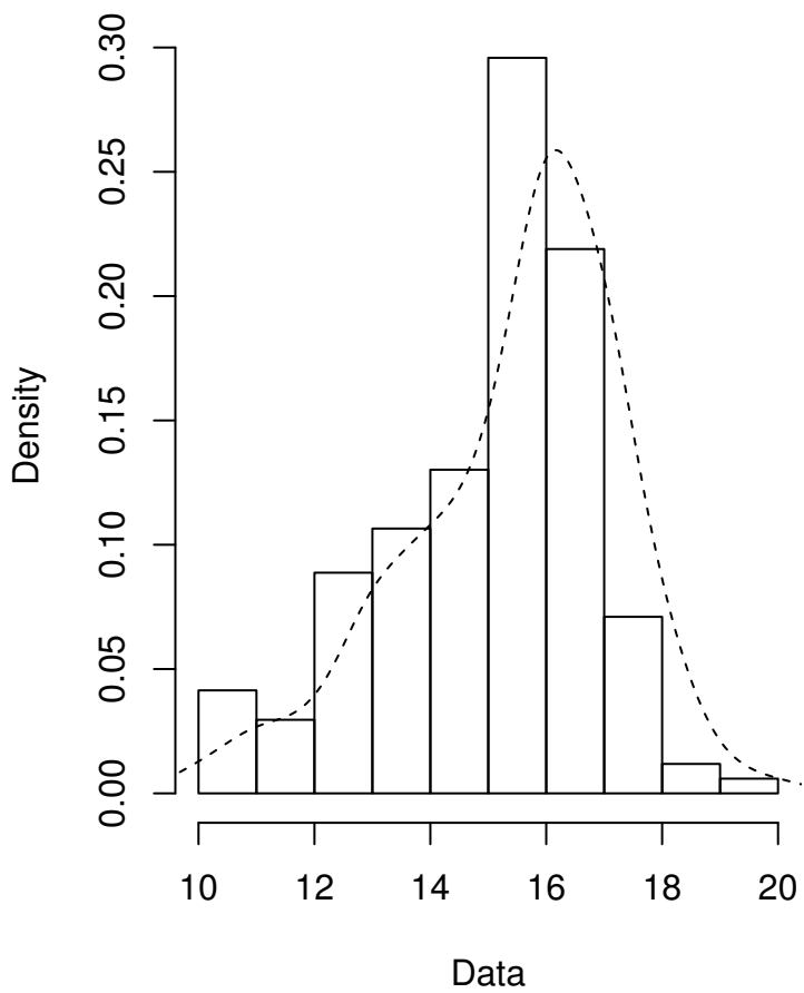
Empirical density
