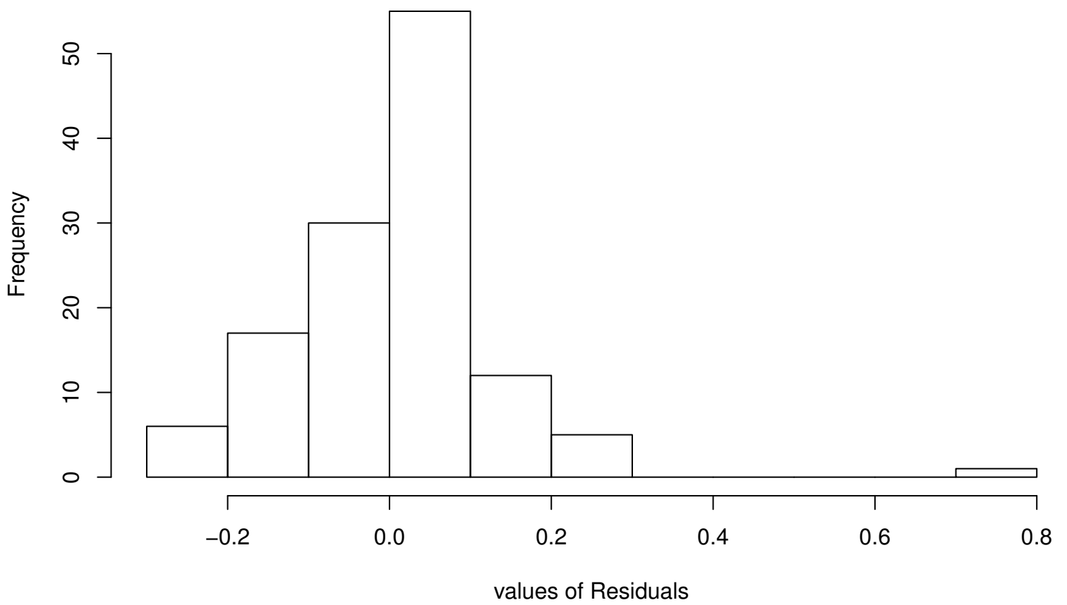
Residual Histogram
