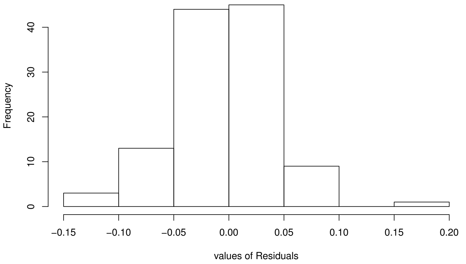
Residual Histogram
