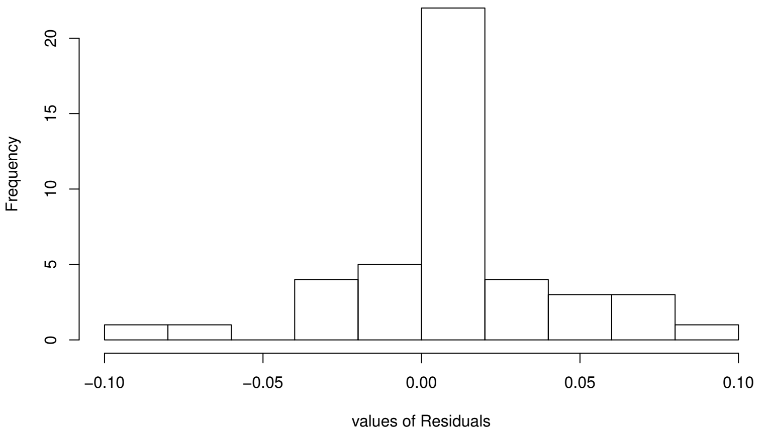
Residual Histogram
