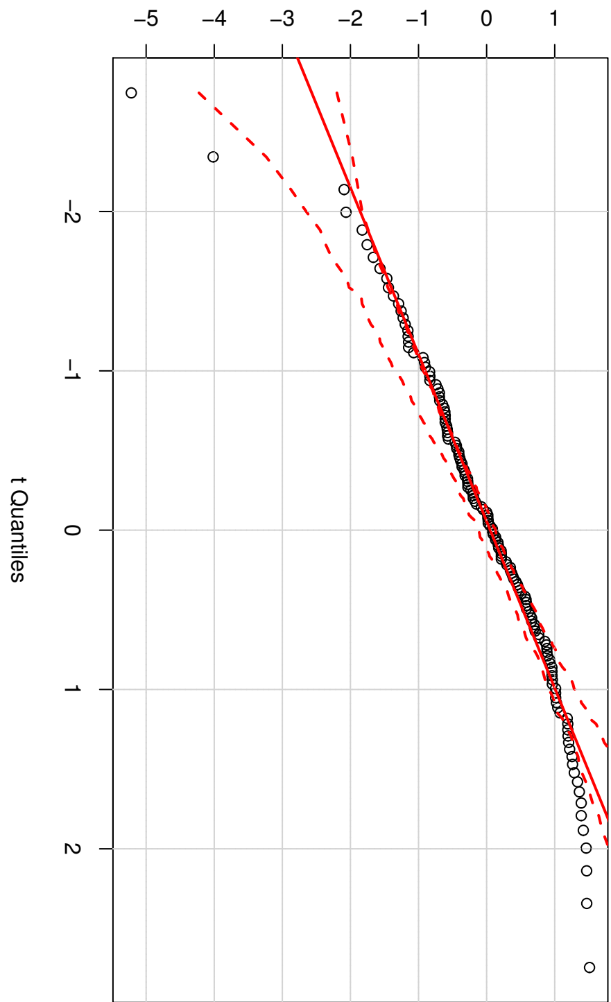
Studentized Residuals(mylm)
