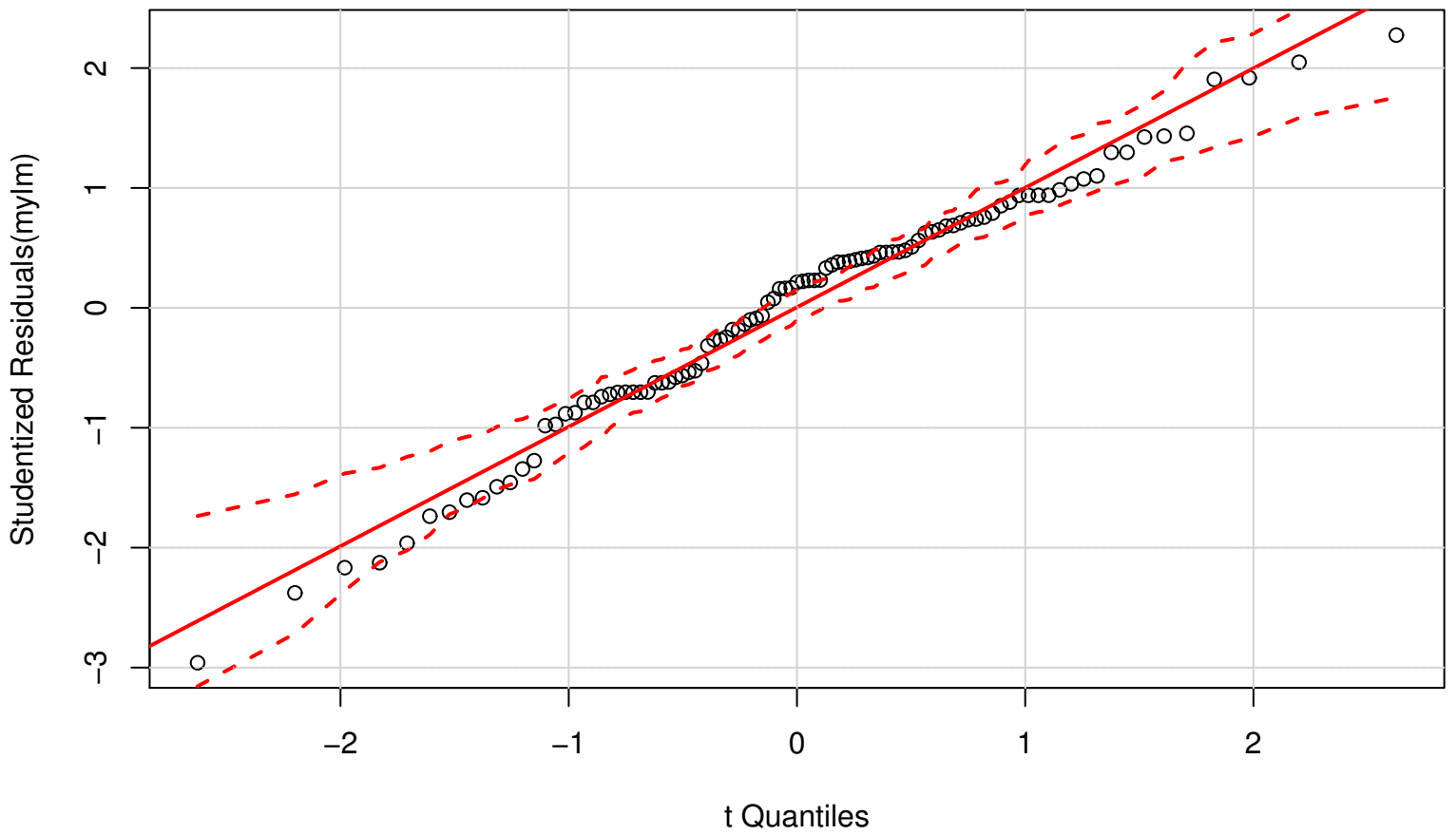
QQ Plot
