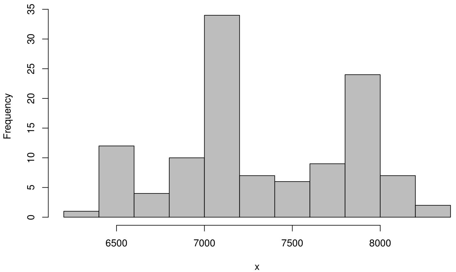
Histogram
