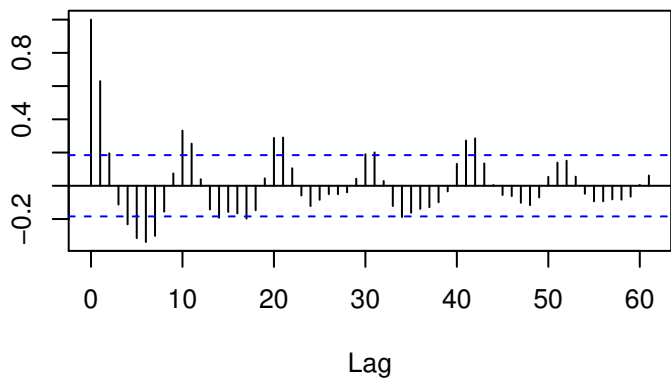
Residual ACF
