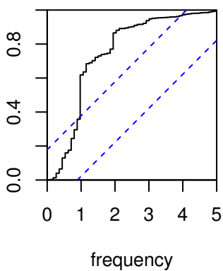
Residual Cumulative Periodogram
