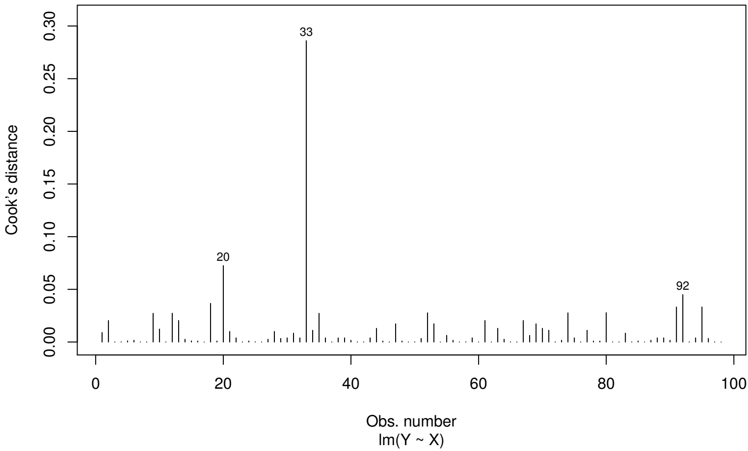
Cook's distance
