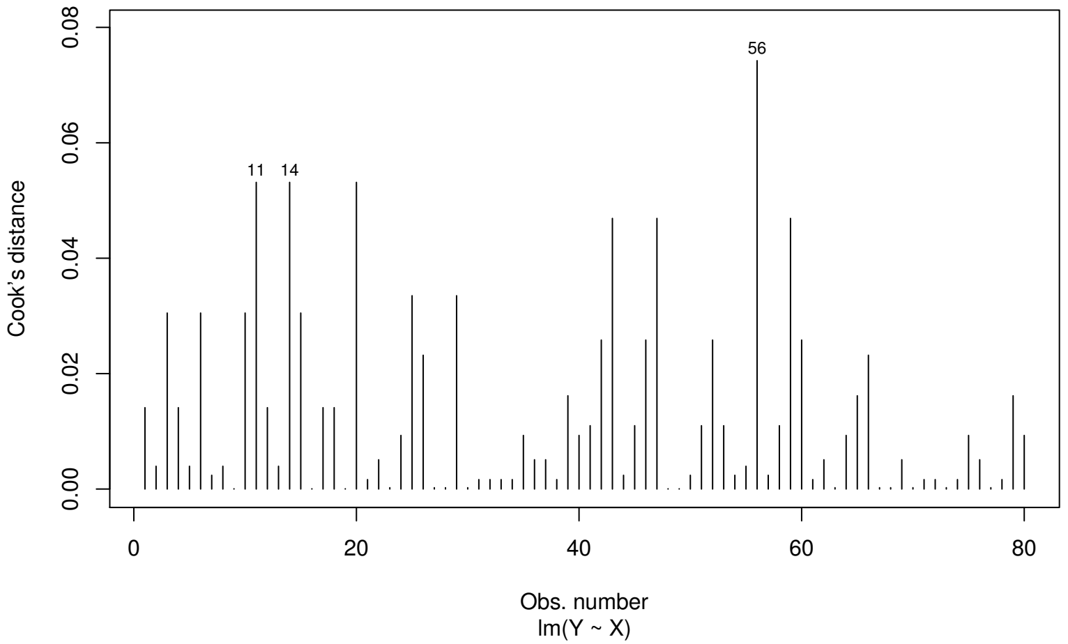
Cook's distance
