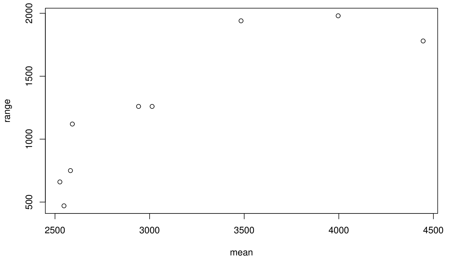
Range–Mean Plot
