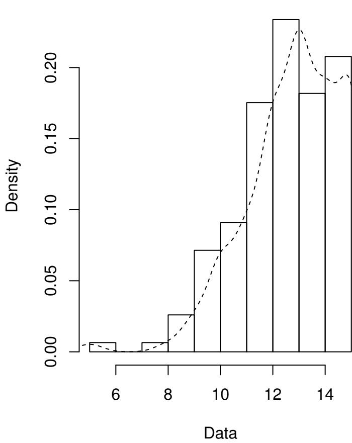
Empirical density
