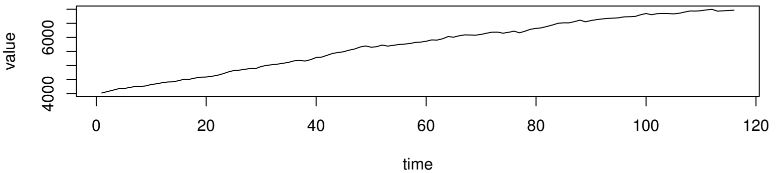
Working Time Series ( \lambda=1 , d=0 , D=0 )
