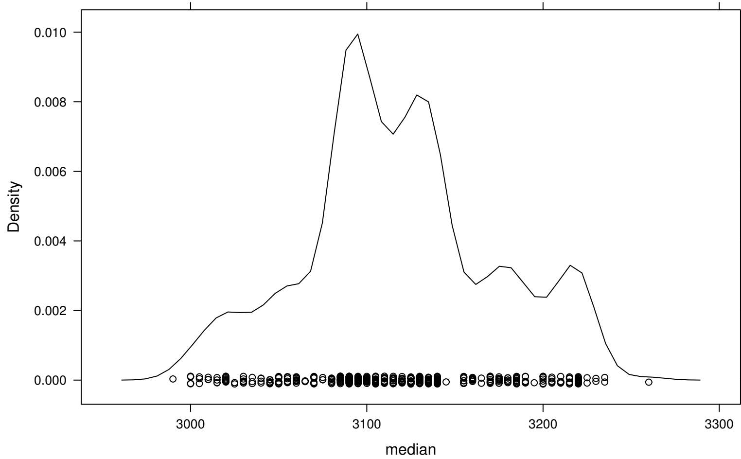
Density Plot
