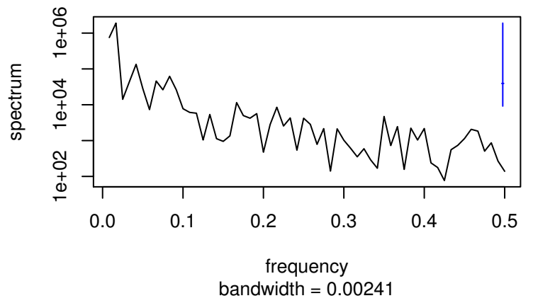
Standardized Residuals
