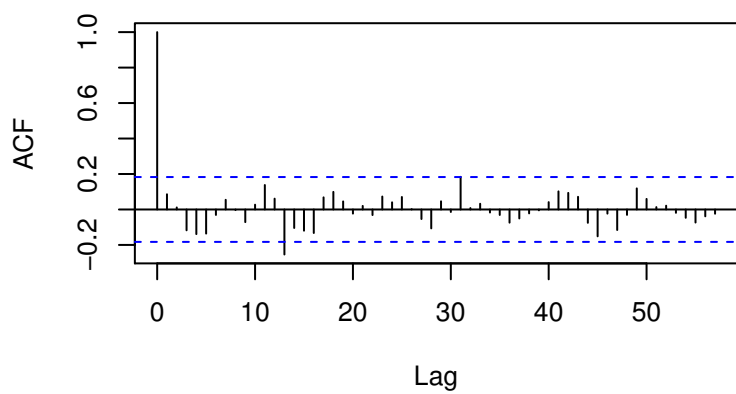
Standardized Residuals
