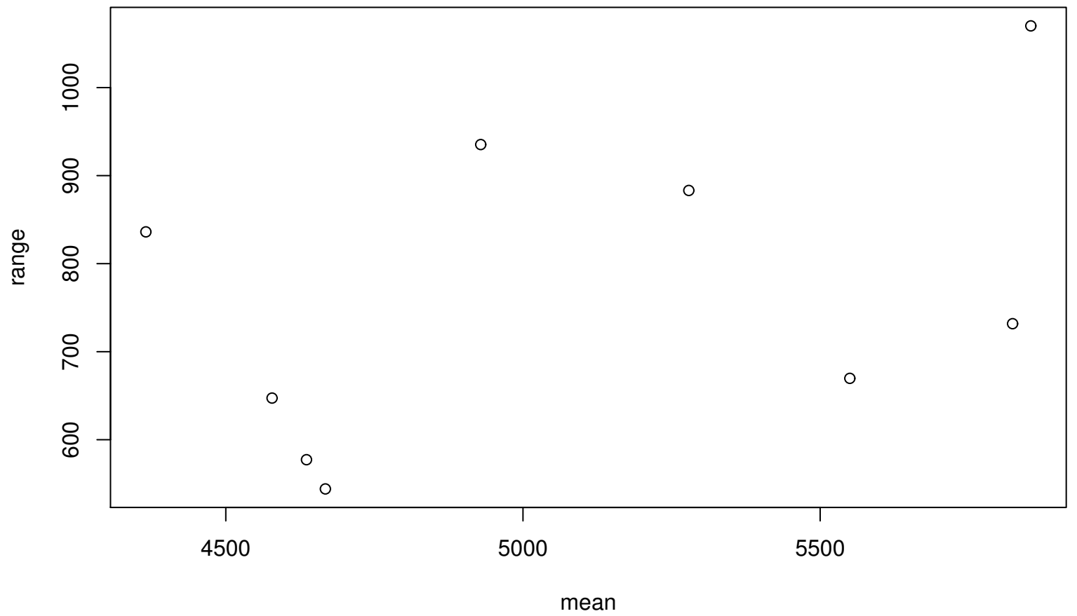
Range–Mean Plot
