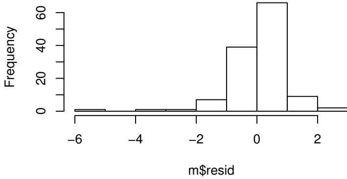
Residual Histogram
