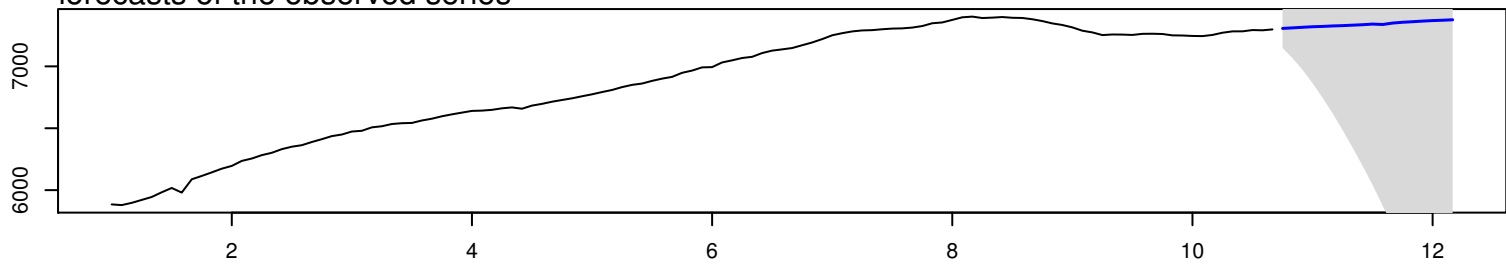
forecasts of the observed series
