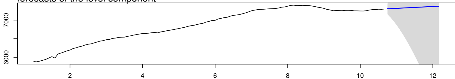
forecasts of the level component
