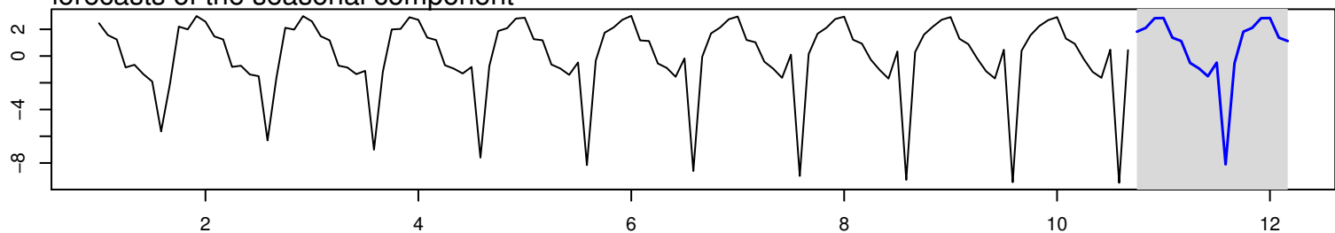
forecasts of the seasonal component
