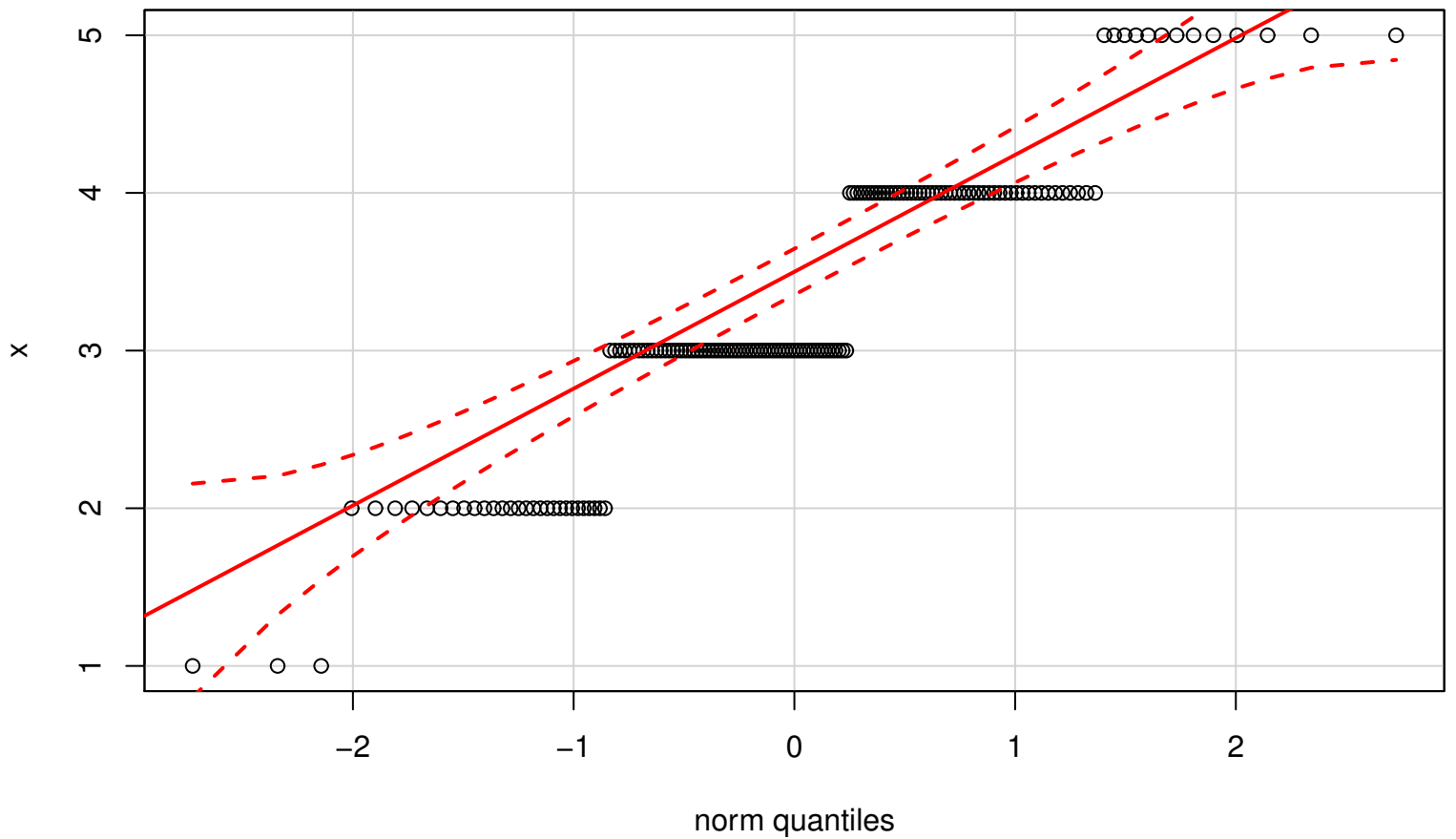
QQplot of variable x
