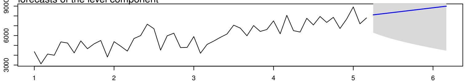
forecasts of the level component
